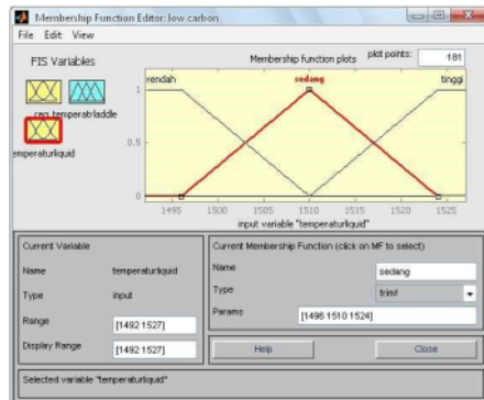
Gambar 4 Input Variabel Liquid Temperature
