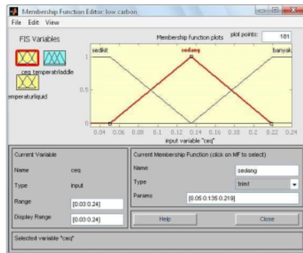
Gambar 3 Input Variabel Carbon Equivalent
