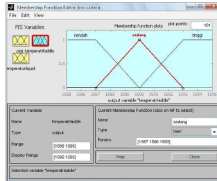
Gambar 5 Output Variabel Ladle Temperature
